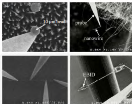
In situ nano-manipulation, electrical and mechanical testing
