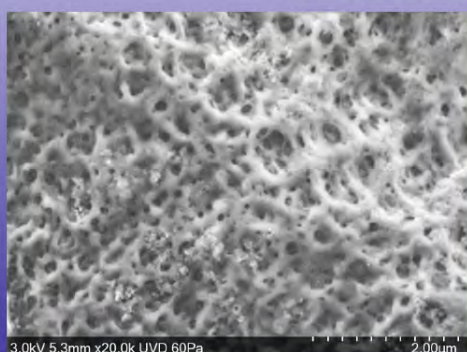
Polymer Filter – Cellulose Esters Pore size of <50nm is confirmed
