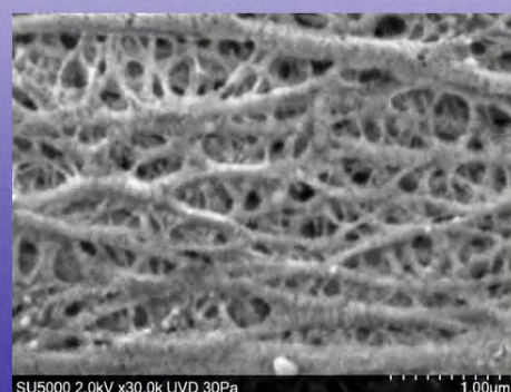
Polymeric Separator in Li battery
